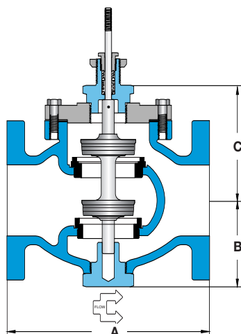
Stem In-to-Close (normally open)
