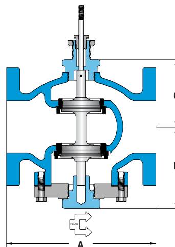
Stem In-to-Open (normally closed)
