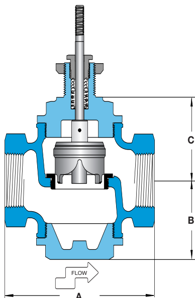
Stem In-to-Close (normally open)
